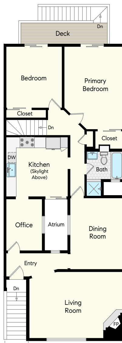
Main Level
